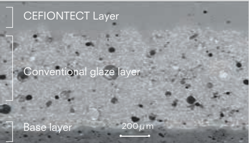
CEFIONTECT toilet micrograph *1Qm=0.001mm
