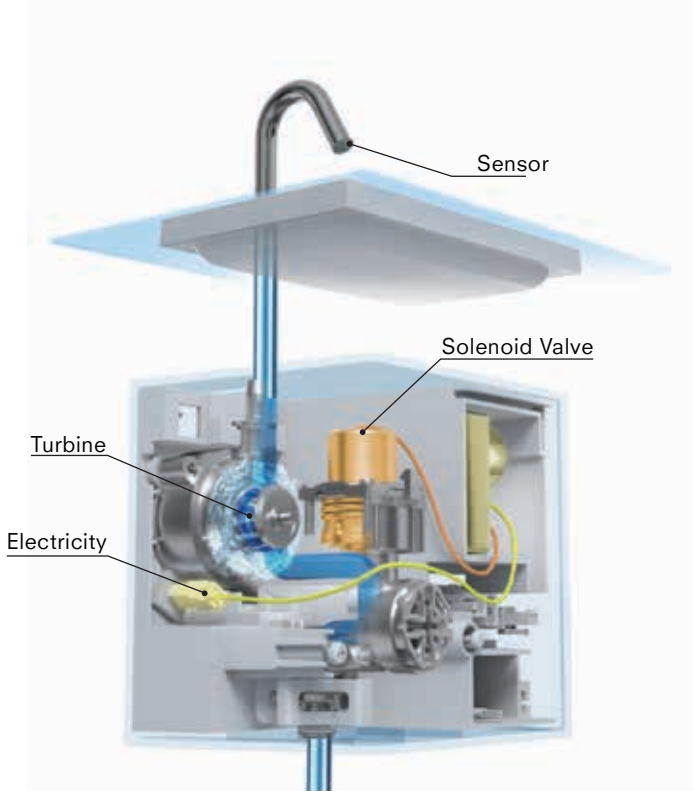
This ECOPOWER touchless faucet uses the flowing water to generate the electricity it needs to operate. There is no need for electrical wiring, making installation and renovation easier.
