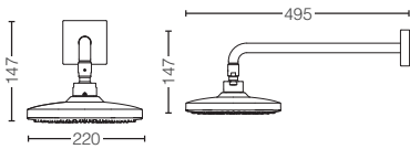
TBW02003BA#BFG Over Head Shower 1 mode, square, 220mm, with pipe Size: 220W x 495D x 147H mm
